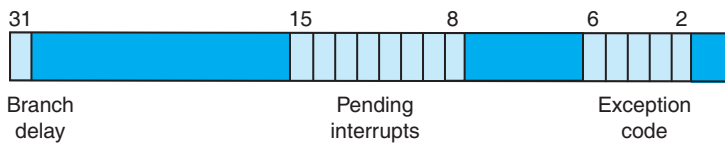
FIGURE A.7.2 The Cause register.
